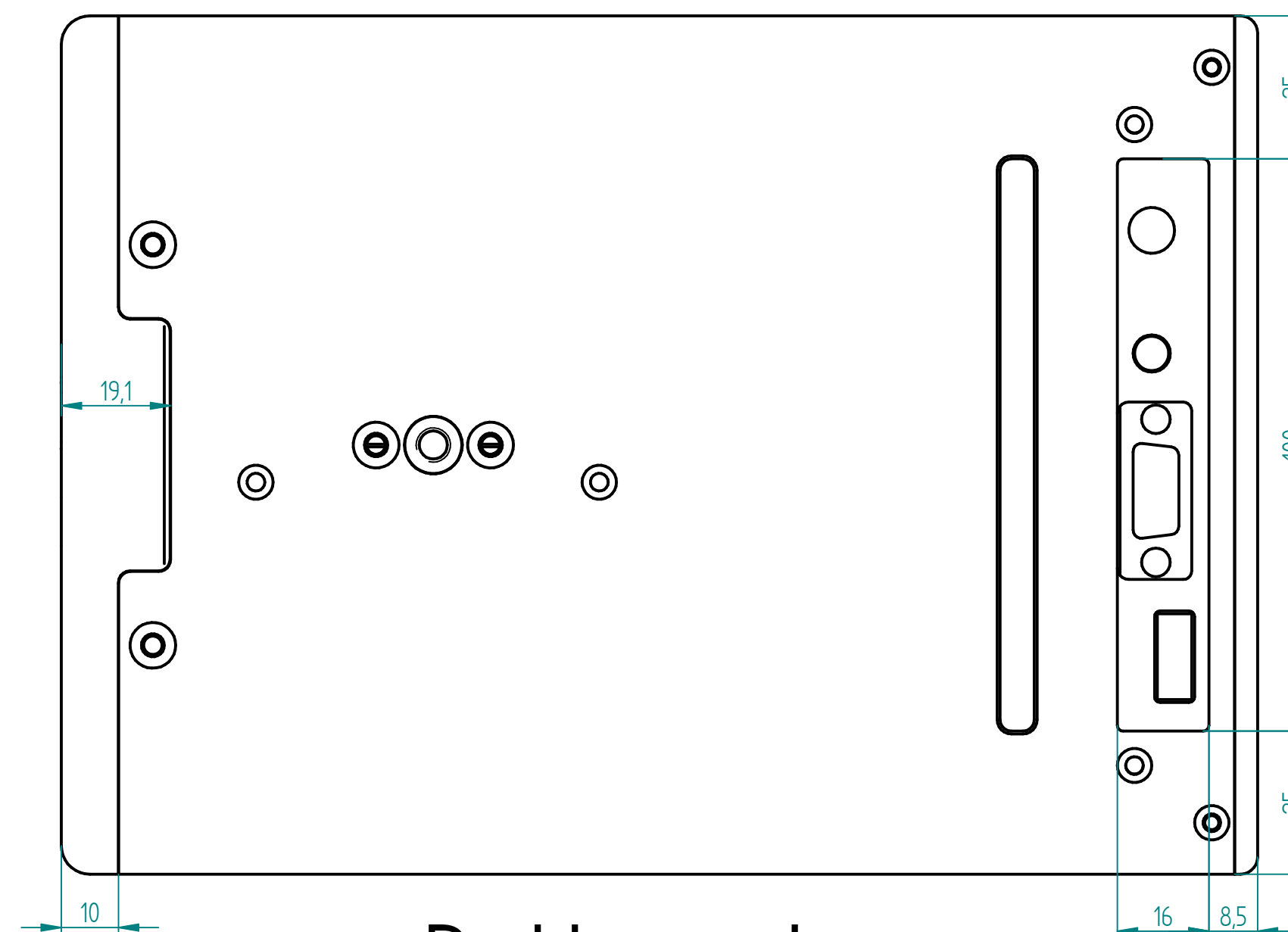
Bottom view
