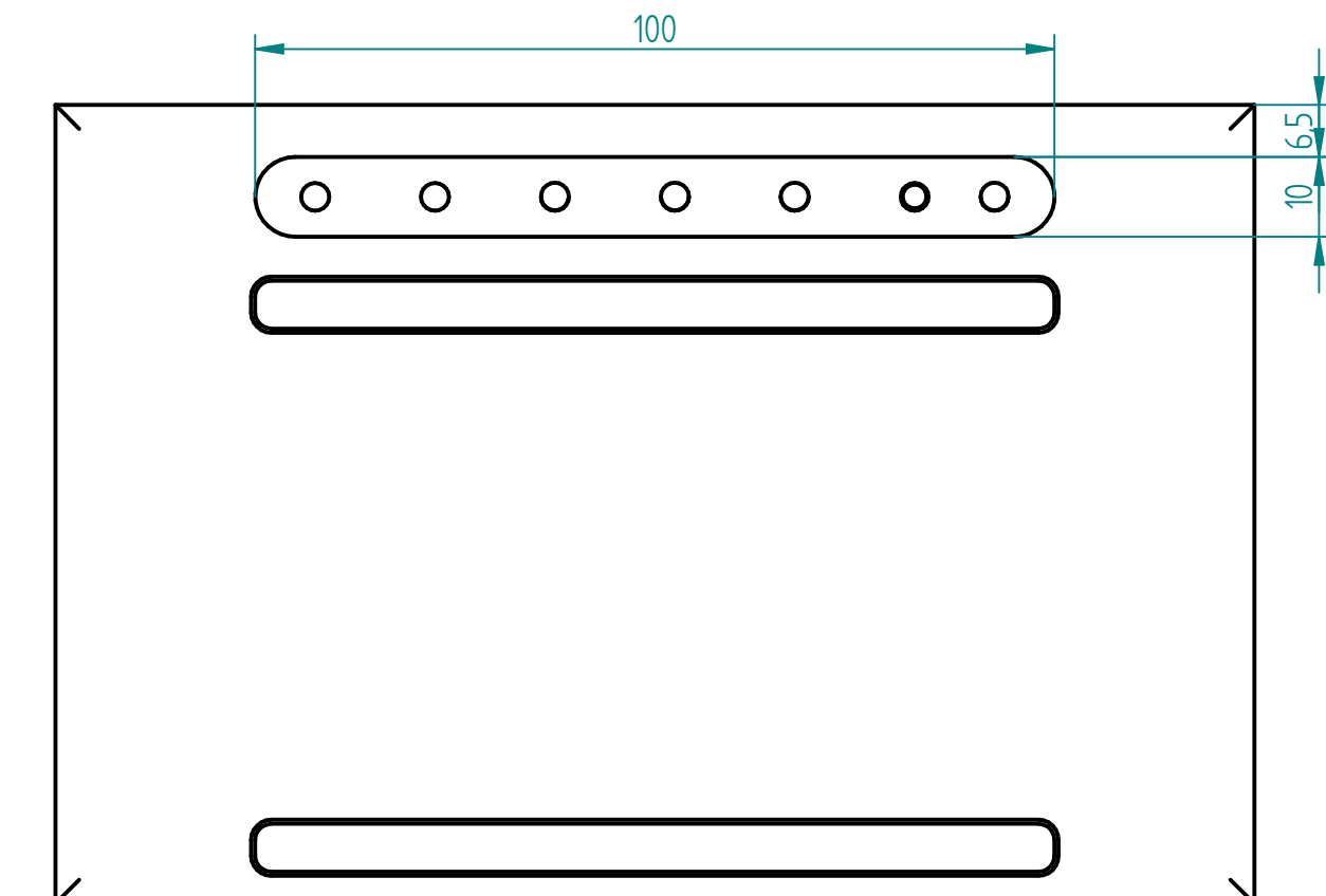
Rear view
